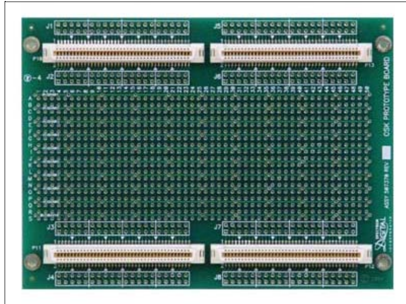
Wire Wrap Prototyping Module for OSKs
